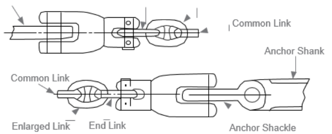
Typical Application
